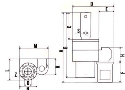
Rotator dimensions
